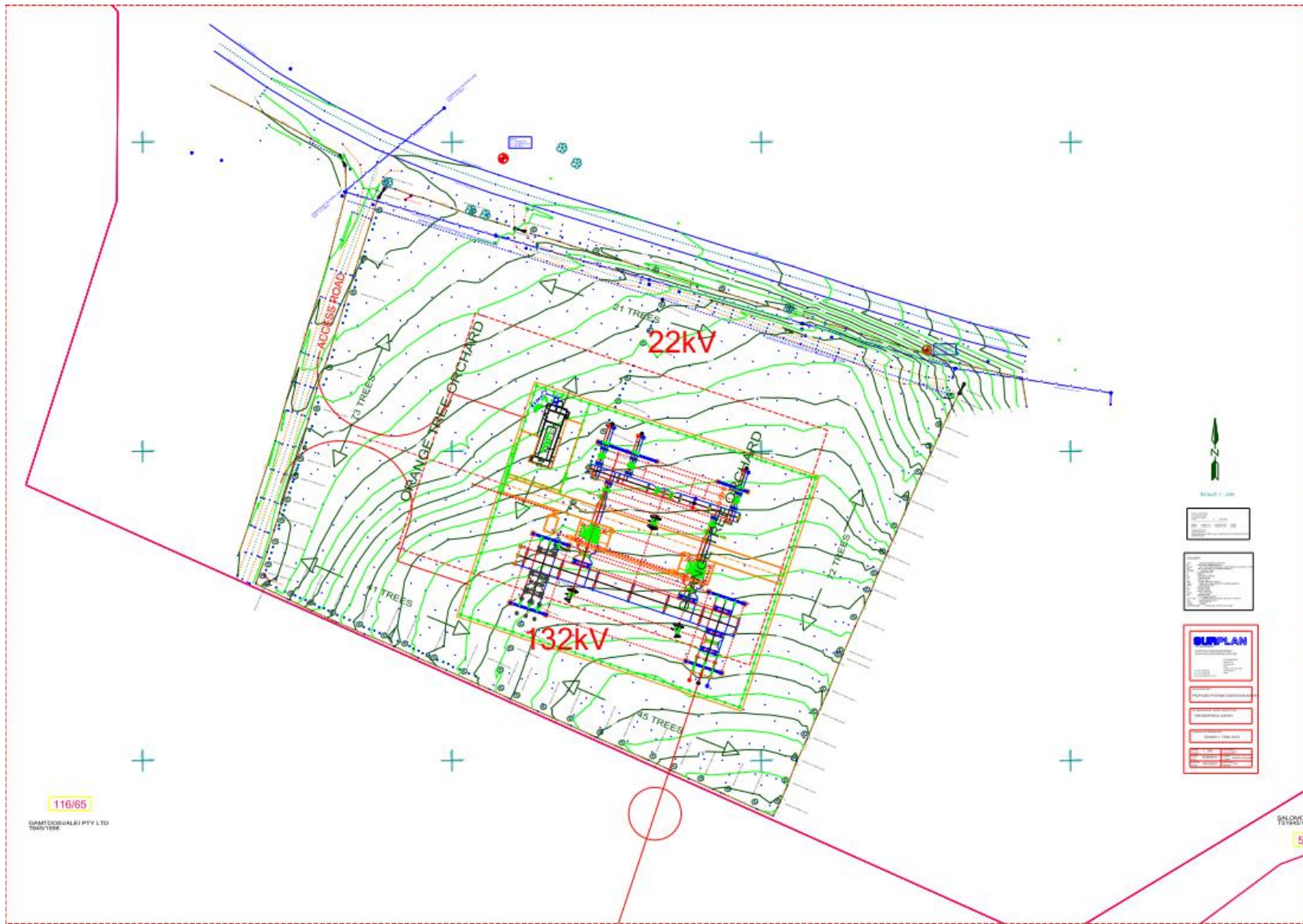
Figure 8: Site layout plan for the Patensie substation
