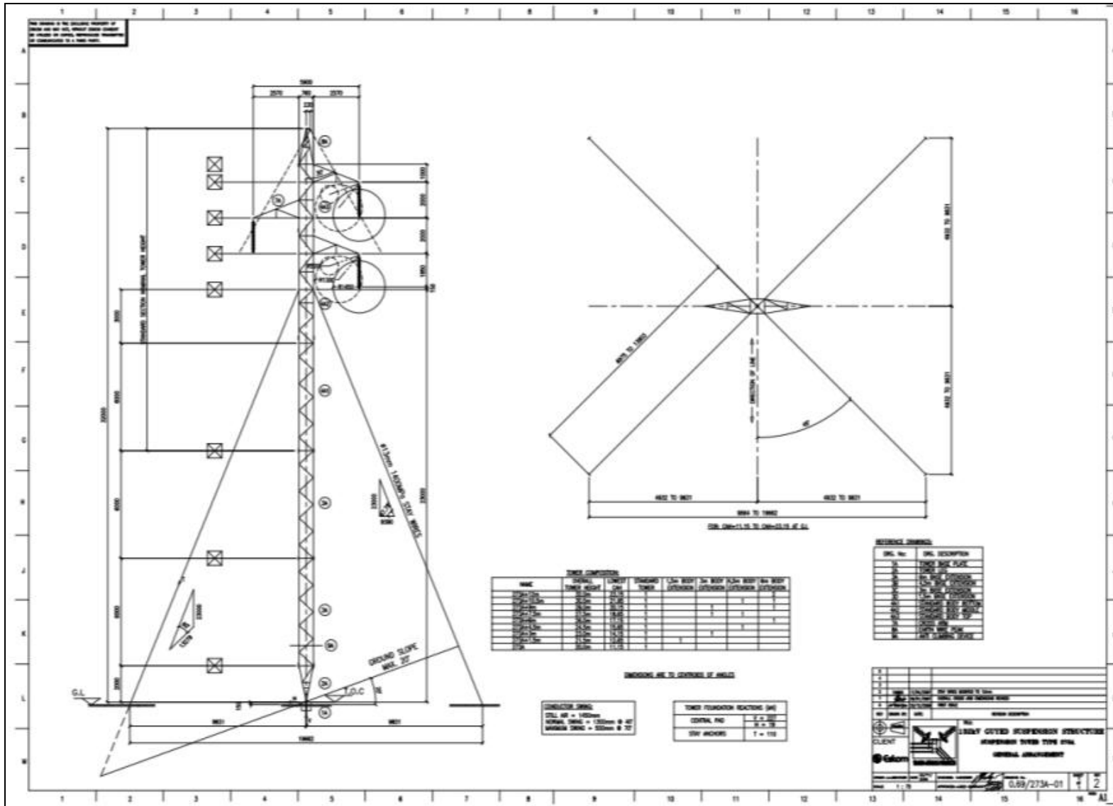
Figure 5: 273A lattice structure
