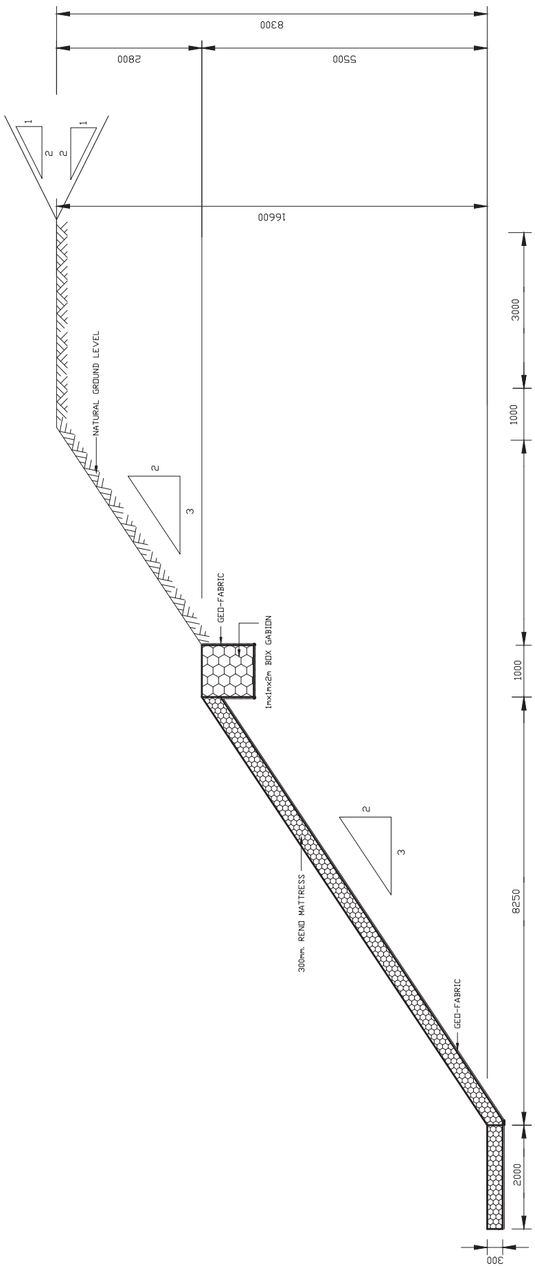
TYPICAL CROSS SECTION OF PROTECTION WORKS SCALE 1:50
